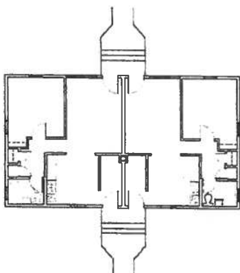
FIRST FLOOR PLAN 4-1 "A"
