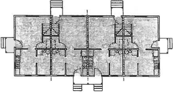
SECOND FLOOR PLAN 4-2 "F"
