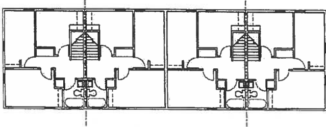
SECOND FLOOR PLAN 4-2 "G"
