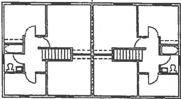
SECOND FLOOR PLAN 4-2 "H"
